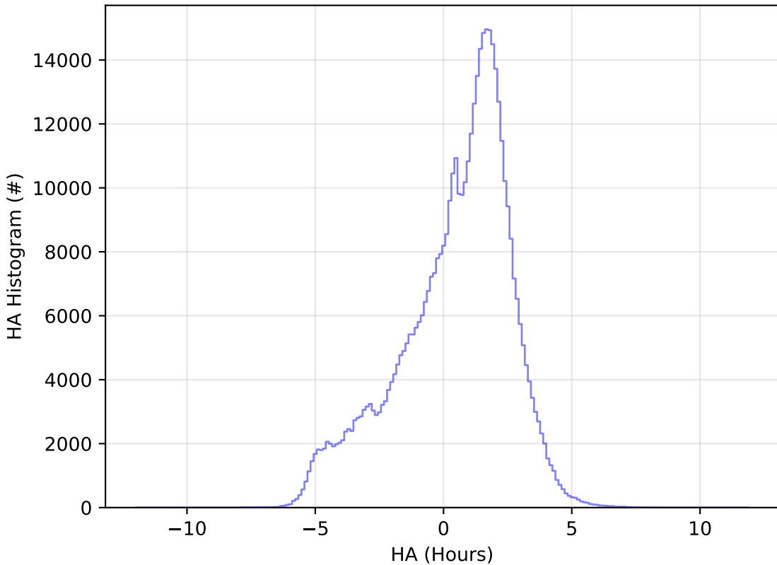
ddf_acor_sf20_lsf0_lsr0_v3.4_10yrs All sky r band: HA Histogram
