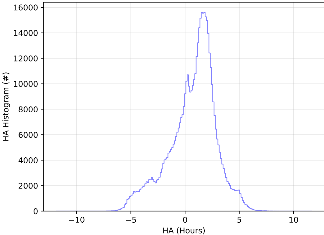
ddf_acor_sf20_lsf0_lsr0_v3.4_10yrs All sky i band: HA Histogram
