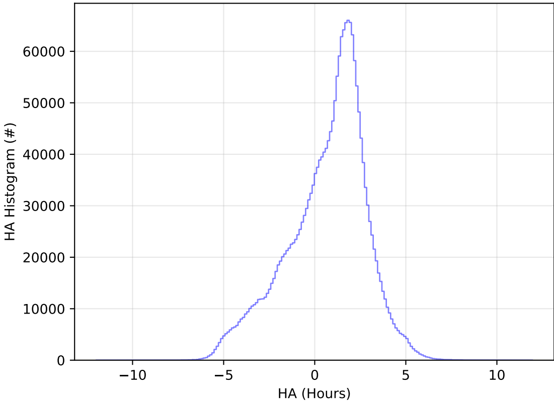
ddf_acor_sf20_lsf0_lsr0_v3.4_10yrs All sky all bands: HA Histogram
