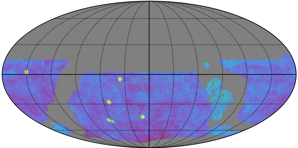
ddf_acor_sf20_lsf0_lsr0_v3.4_10yrs gri WFD: Fraction of visits in pairs (10-60 min)
