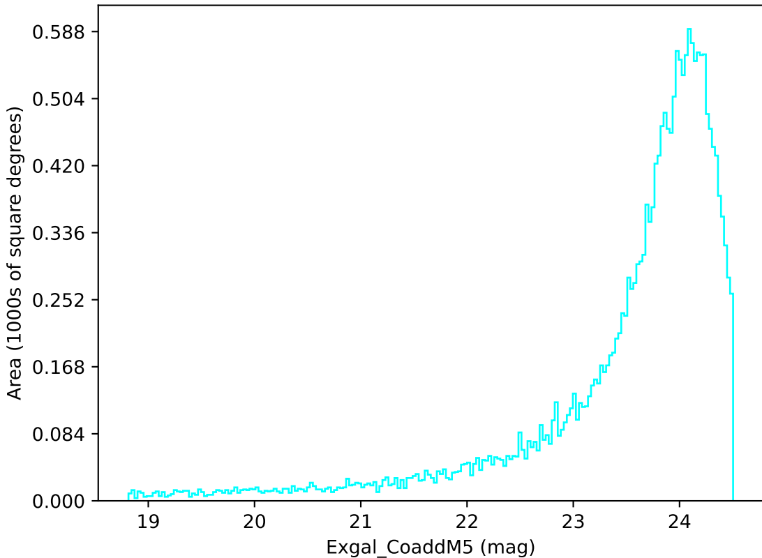
ddf_acor_sf20_lsf0_lsr0_v3.4_10yrs Yr 1 u band: Exgal_CoaddM5
