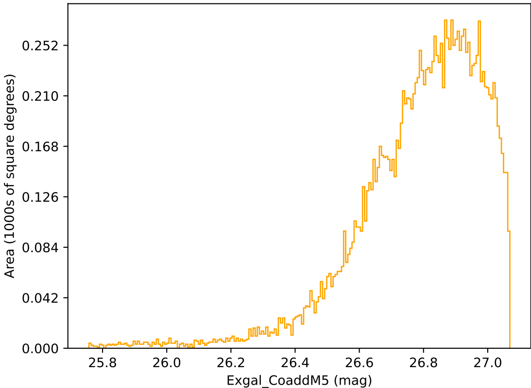
ddf_acor_sf20_lsf0_lsr0_v3.4_10yrs WFD r band: Exgal_CoaddM5
