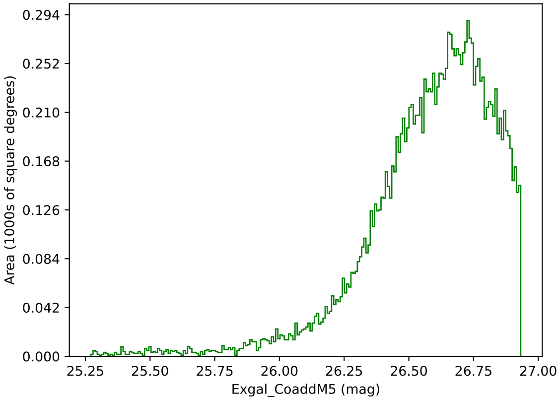
ddf_acor_sf20_lsf0_lsr0_v3.4_10yrs WFD g band: Exgal_CoaddM5
