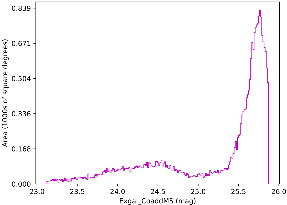
ddf_acor_sf20_lsf0_lsr0_v3.4_10yrs All sky z band: Exgal_CoaddM5
