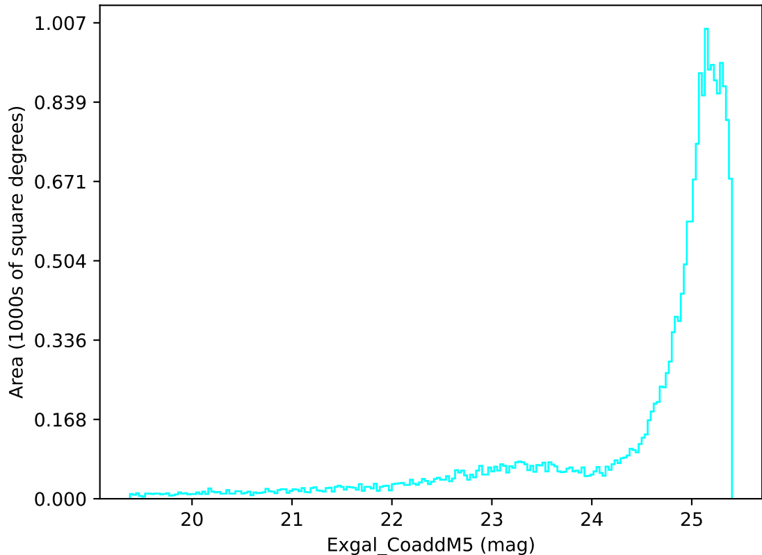
ddf_acor_sf20_lsf0_lsr0_v3.4_10yrs All sky u band: Exgal_CoaddM5
