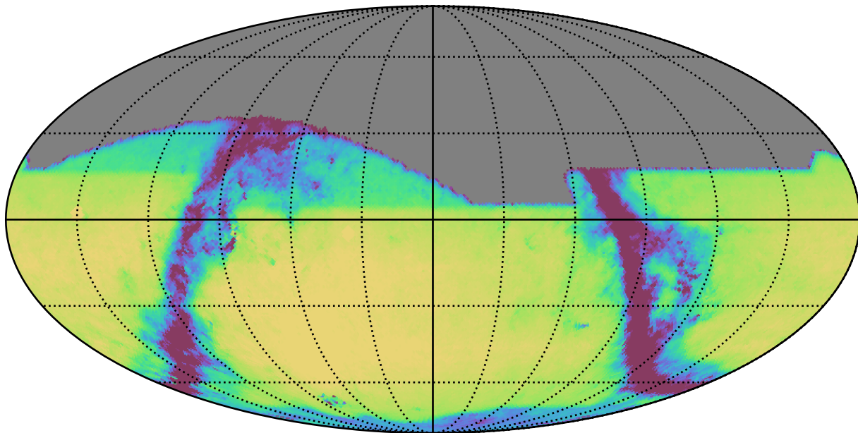
ddf_acor_sf20_lsf0_lsr0_v3.4_10yrs All sky r band: Exgal_CoaddM5
