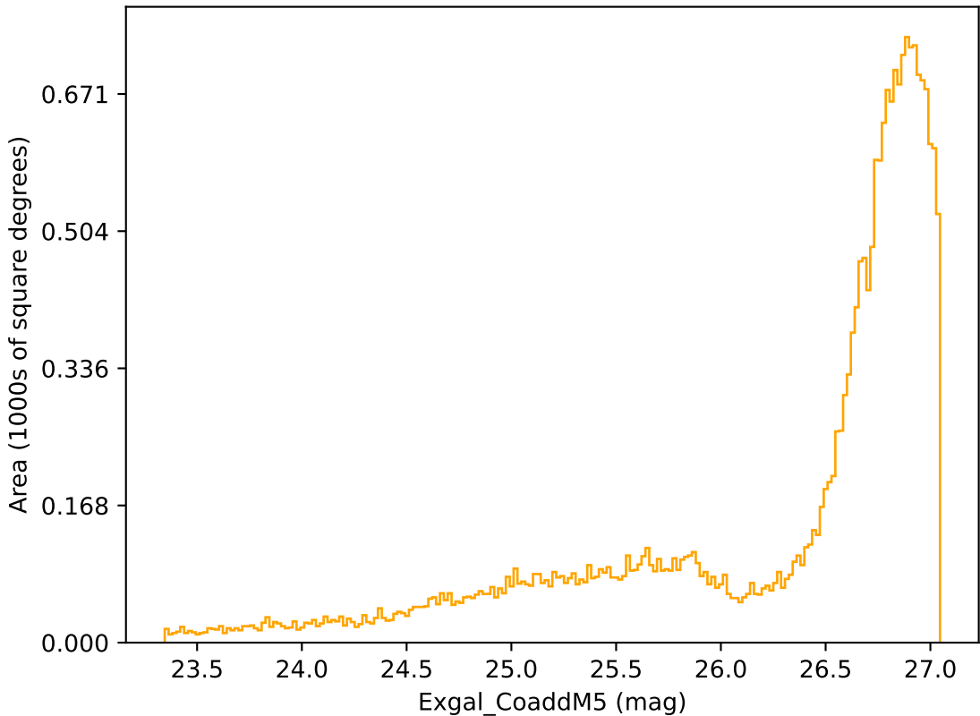
ddf_acor_sf20_lsf0_lsr0_v3.4_10yrs All sky r band: Exgal_CoaddM5
