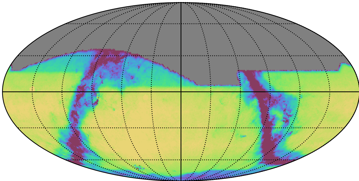
ddf_acor_sf20_lsf0_lsr0_v3.4_10yrs All sky i band: Exgal_CoaddM5
