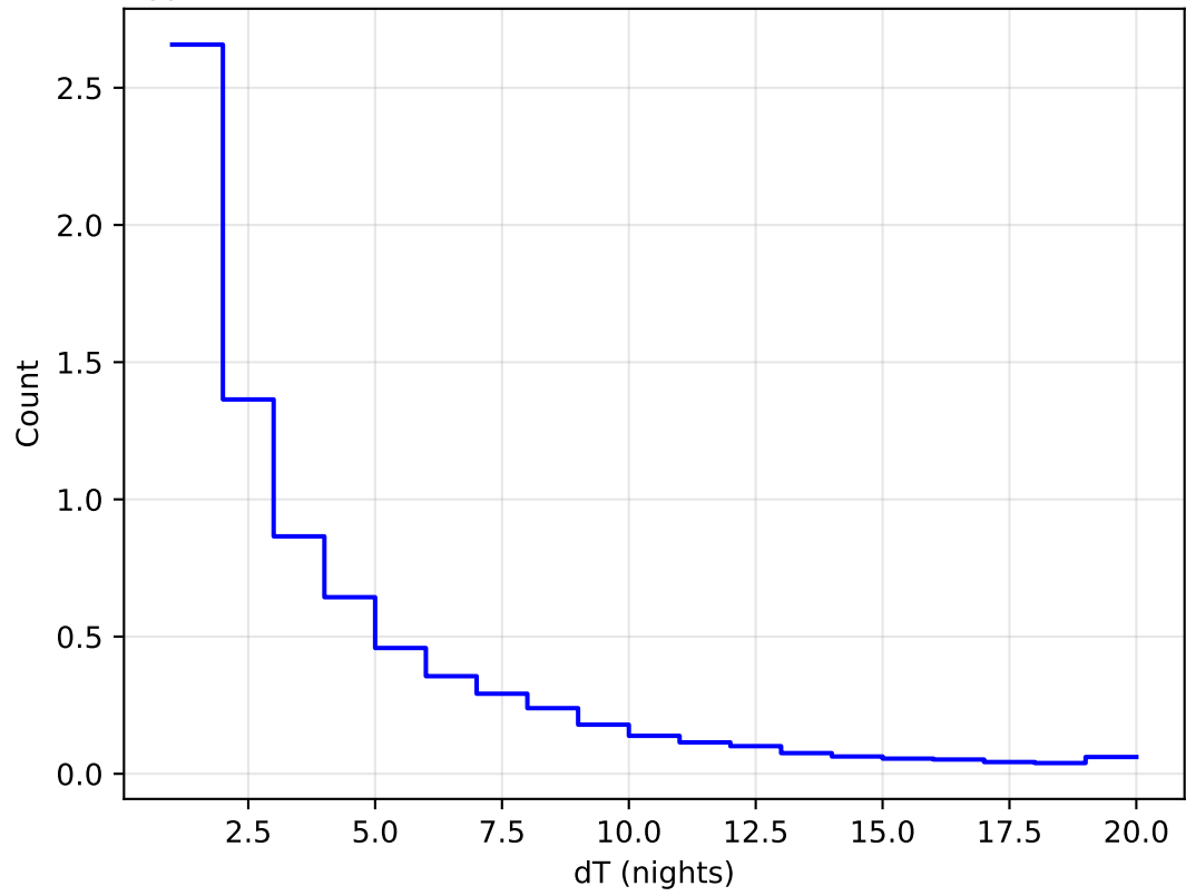
ddf_acor_sf20_lsf0_lsr0_v3.4_10yrs WFD all bands: DeltaNight Histogram
