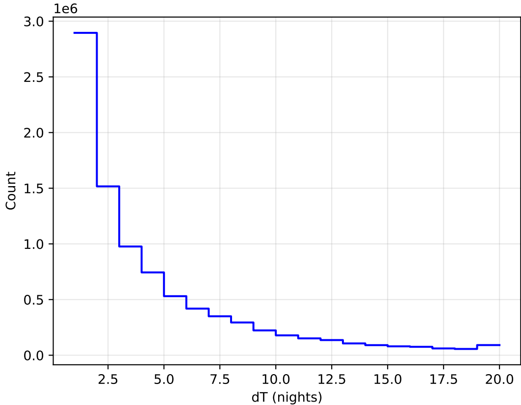
ddf_acor_sf20_lsf0_lsr0_v3.4_10yrs All sky all bands: DeltaNight Histogram
