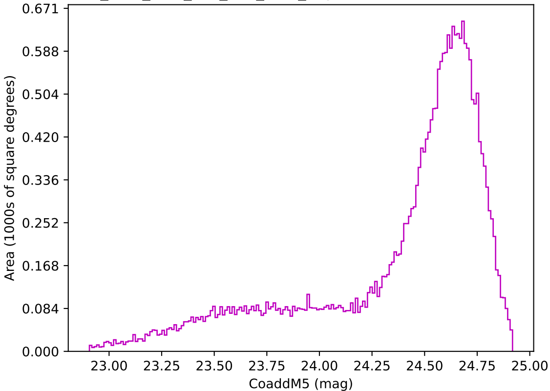
ddf_acor_sf20_lsf0_lsr0_v3.4_10yrs Yr 1 z band: CoaddM5
