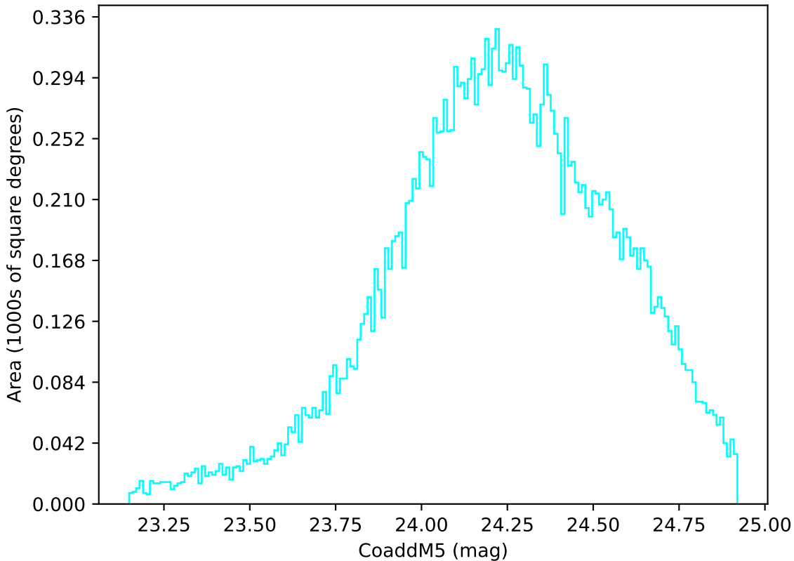
ddf_acor_sf20_lsf0_lsr0_v3.4_10yrs Yr 1 u band: CoaddM5
