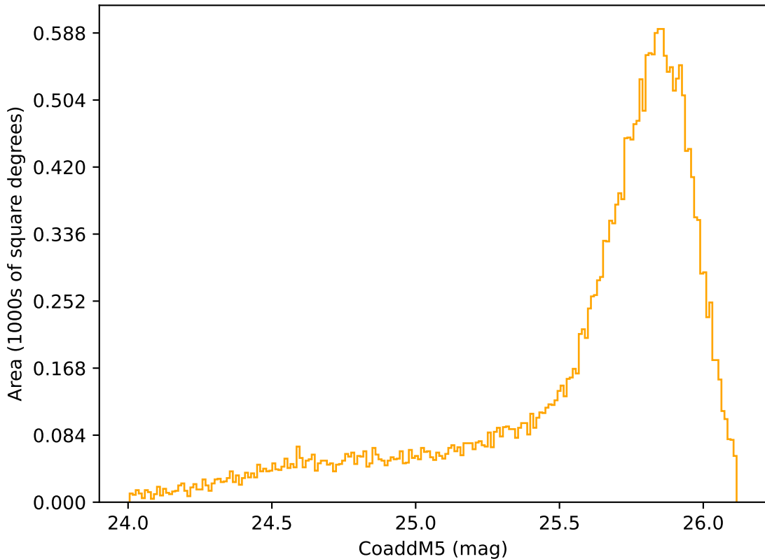
ddf_acor_sf20_lsf0_lsr0_v3.4_10yrs Yr 1 r band: CoaddM5
