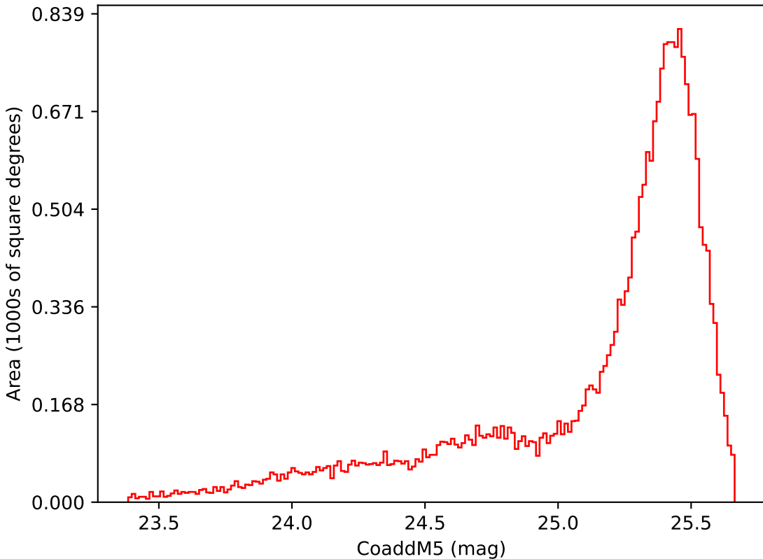
ddf_acor_sf20_lsf0_lsr0_v3.4_10yrs Yr 1 i band: CoaddM5
