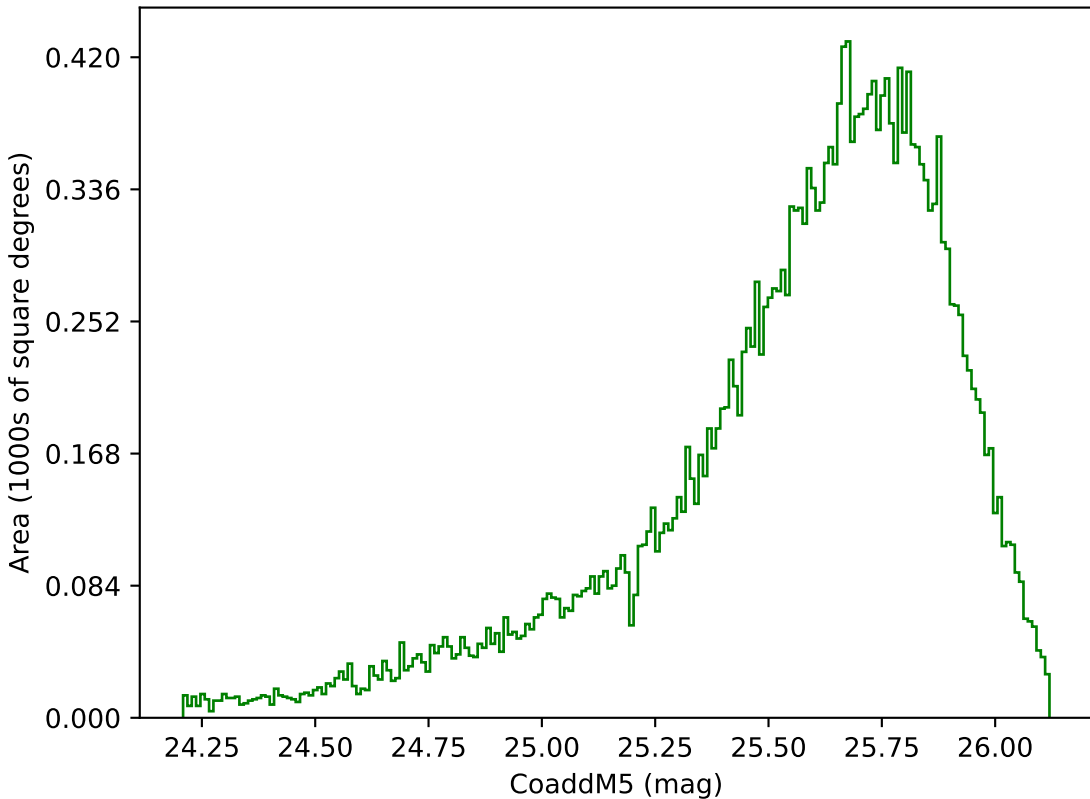
ddf_acor_sf20_lsf0_lsr0_v3.4_10yrs Yr 1 g band: CoaddM5
