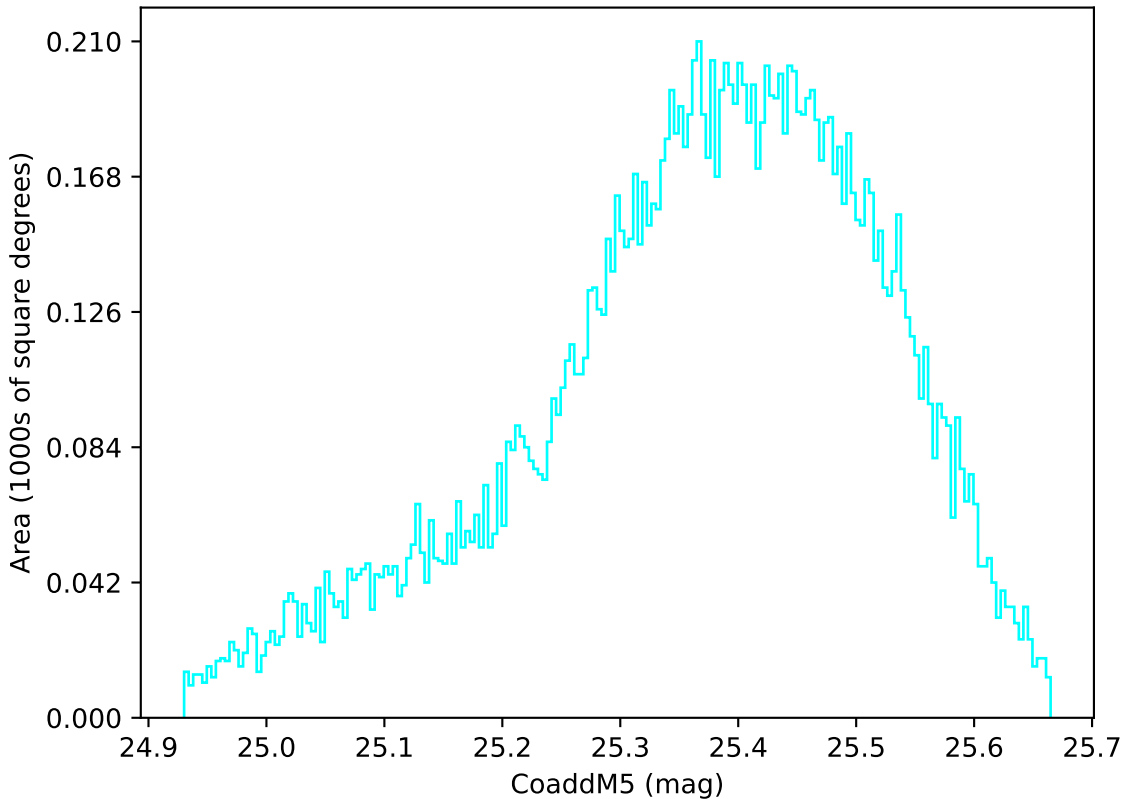
ddf_acor_sf20_lsf0_lsr0_v3.4_10yrs WFD u band: CoaddM5
