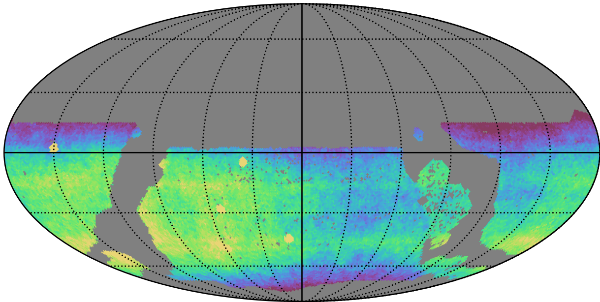
ddf_acor_sf20_lsf0_lsr0_v3.4_10yrs WFD r band: CoaddM5
