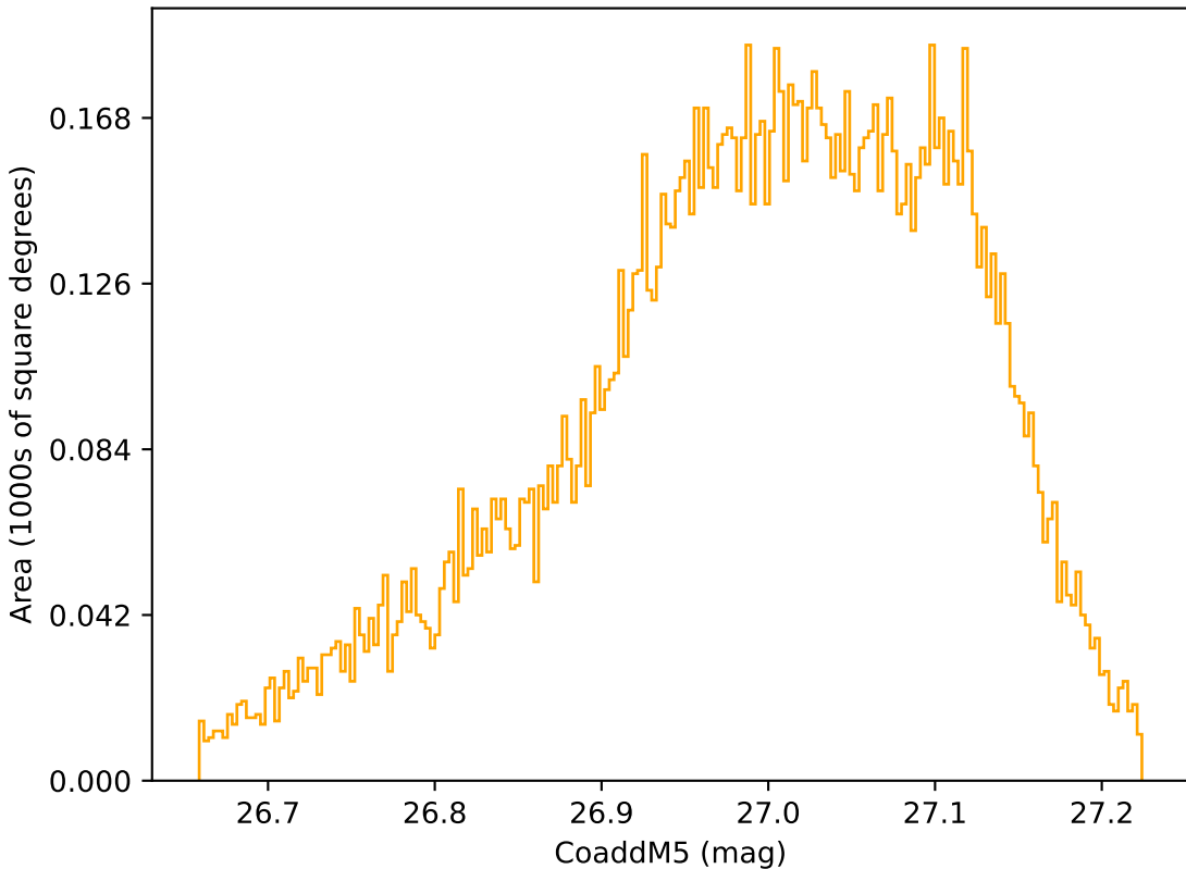
ddf_acor_sf20_lsf0_lsr0_v3.4_10yrs WFD r band: CoaddM5
