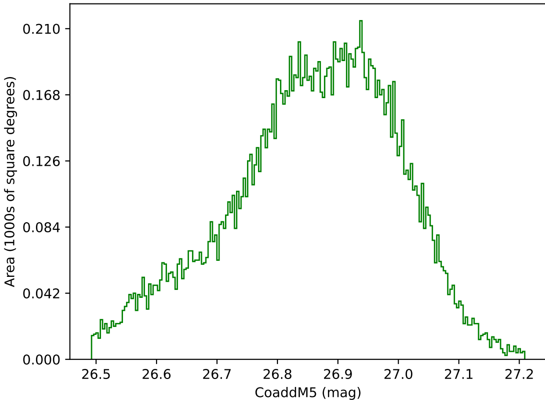
ddf_acor_sf20_lsf0_lsr0_v3.4_10yrs WFD g band: CoaddM5
