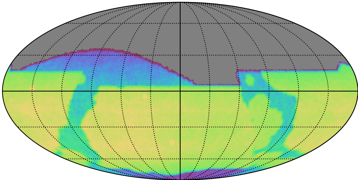
ddf_acor_sf20_lsf0_lsr0_v3.4_10yrs All sky z band: CoaddM5
