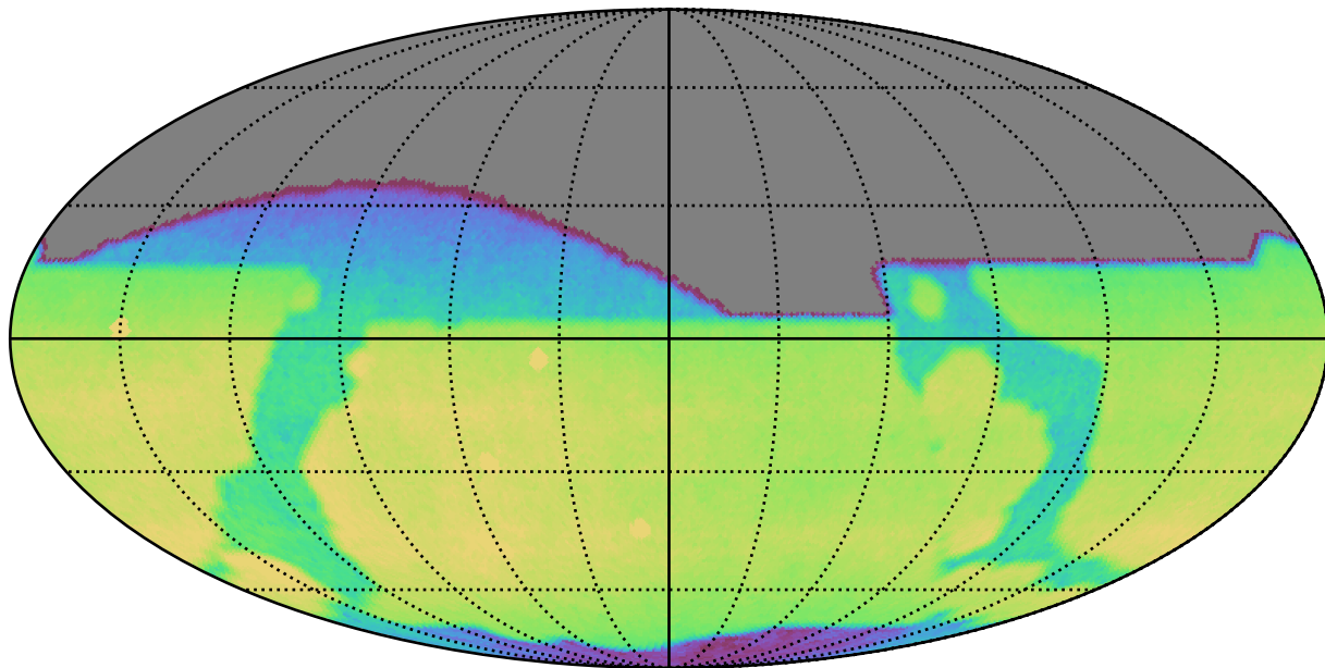
ddf_acor_sf20_lsf0_lsr0_v3.4_10yrs All sky r band: CoaddM5
