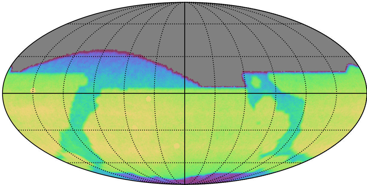
ddf_acor_sf20_lsf0_lsr0_v3.4_10yrs All sky i band: CoaddM5
