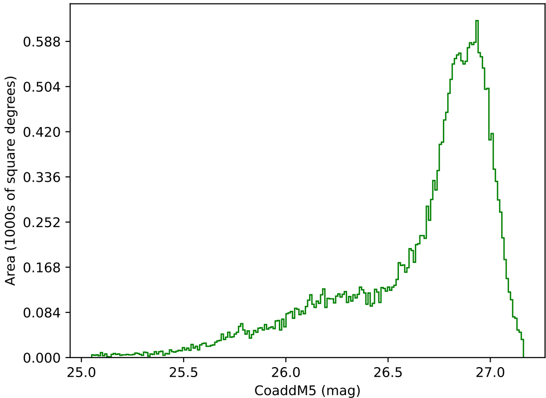
ddf_acor_sf20_lsf0_lsr0_v3.4_10yrs All sky g band: CoaddM5
