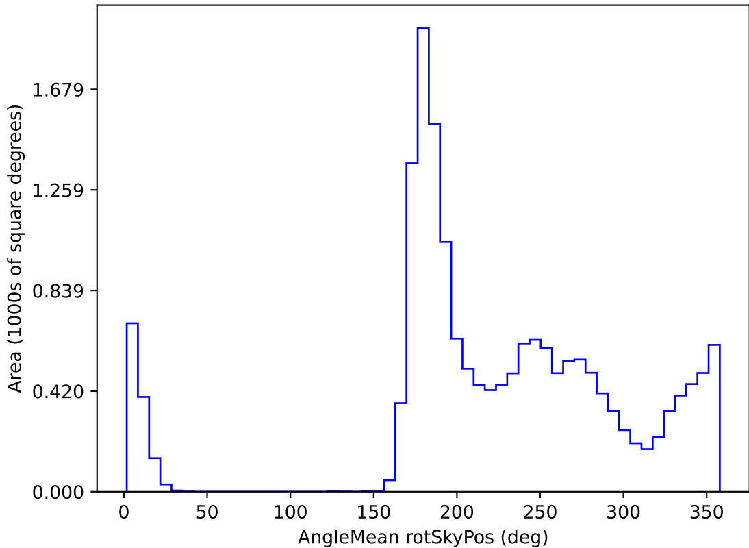
ddf_acor_sf20_lsf0_lsr0_v3.4_10yrs WFD y band: AngleMean rotSkyPos
