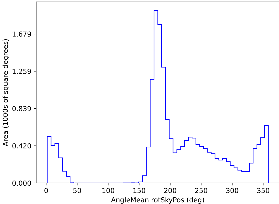
ddf_acor_sf20_lsf0_lsr0_v3.4_10yrs WFD r band: AngleMean rotSkyPos
