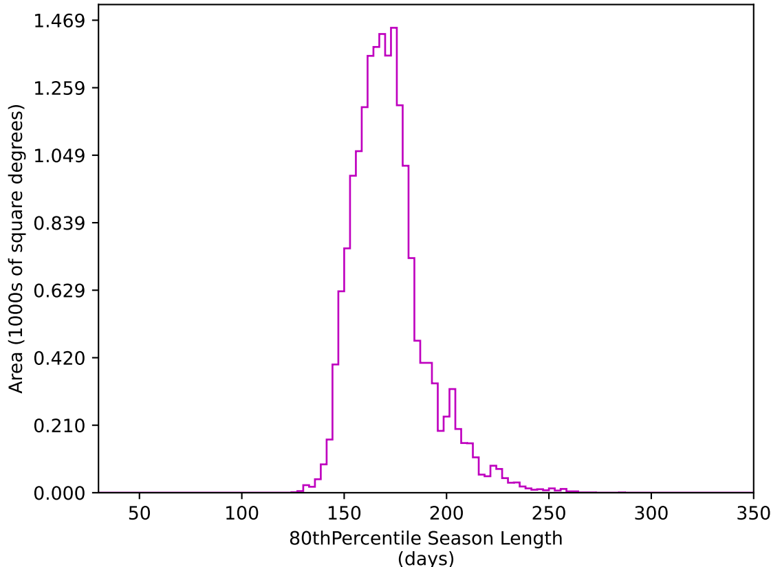
ddf_acor_sf20_lsf0_lsr0_v3.4_10yrs WFD z band: 80thPercentile Season Length
