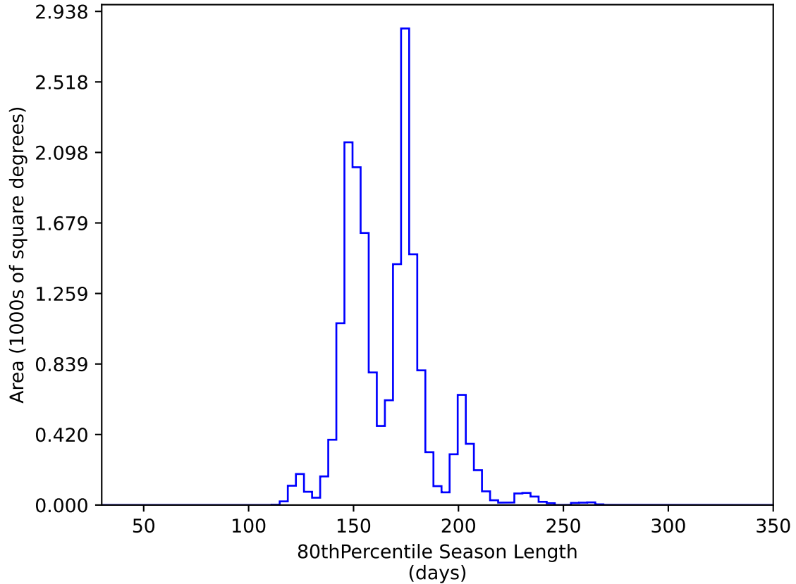
ddf_acor_sf20_lsf0_lsr0_v3.4_10yrs WFD y band: 80thPercentile Season Length
