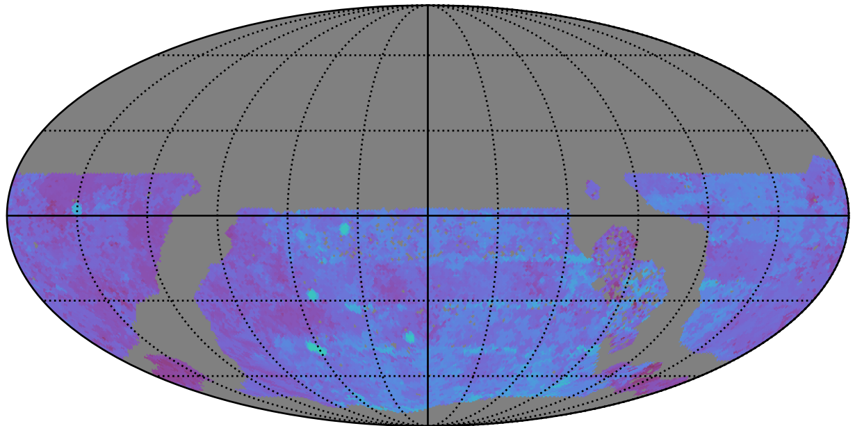
ddf_acor_sf20_lsf0_lsr0_v3.4_10yrs WFD u band: 80thPercentile Season Length
