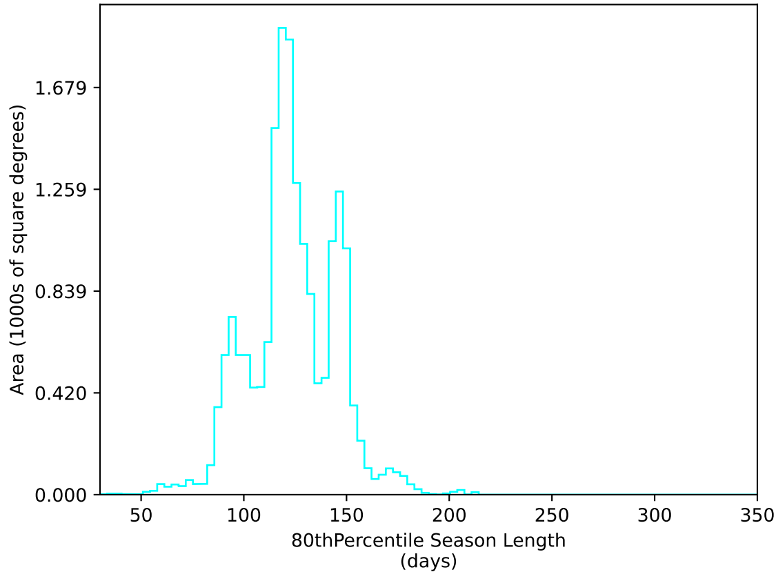
ddf_acor_sf20_lsf0_lsr0_v3.4_10yrs WFD u band: 80thPercentile Season Length
