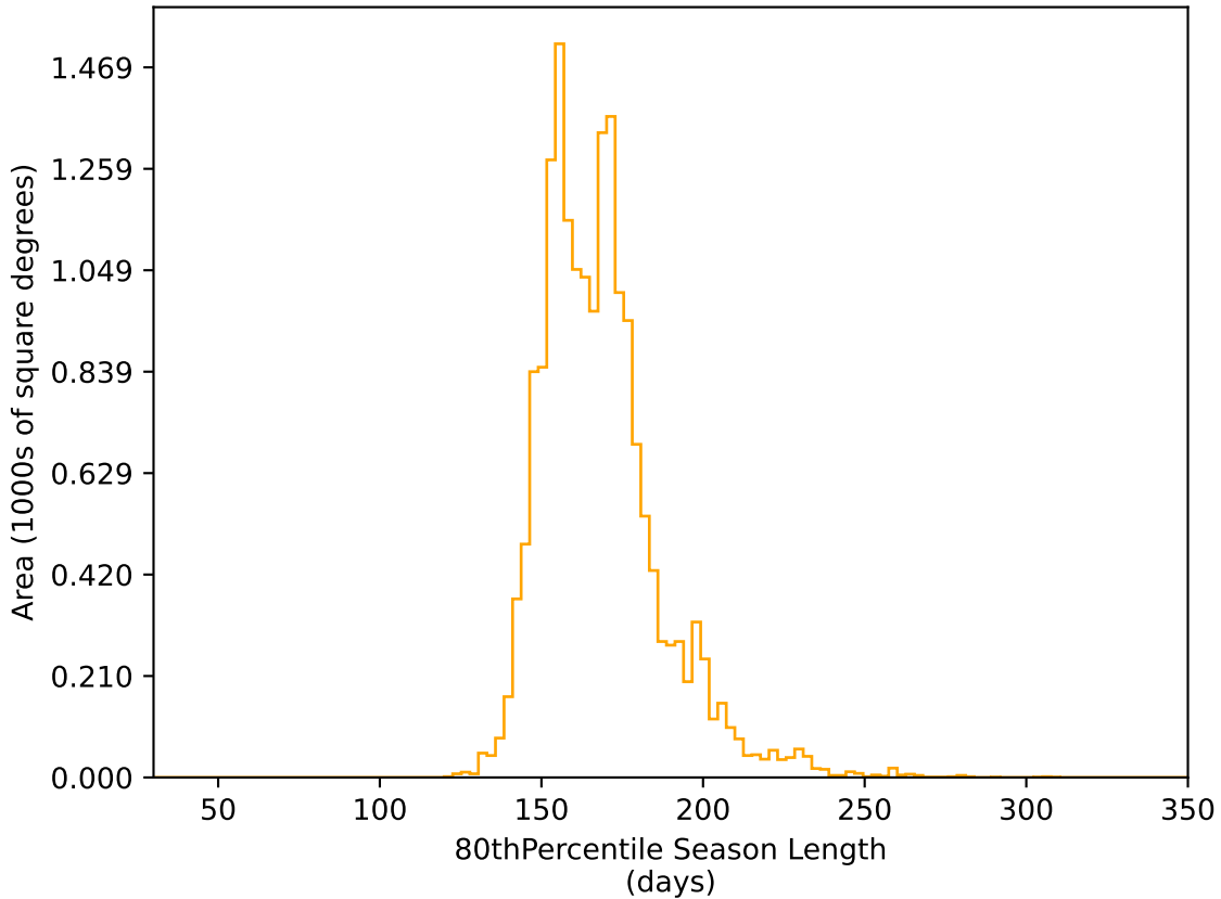
ddf_acor_sf20_lsf0_lsr0_v3.4_10yrs WFD r band: 80thPercentile Season Length
