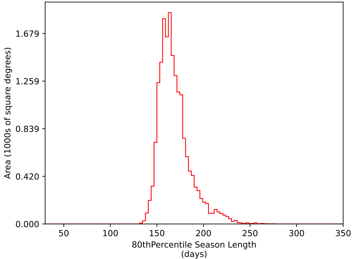
ddf_acor_sf20_lsf0_lsr0_v3.4_10yrs WFD i band: 80thPercentile Season Length
