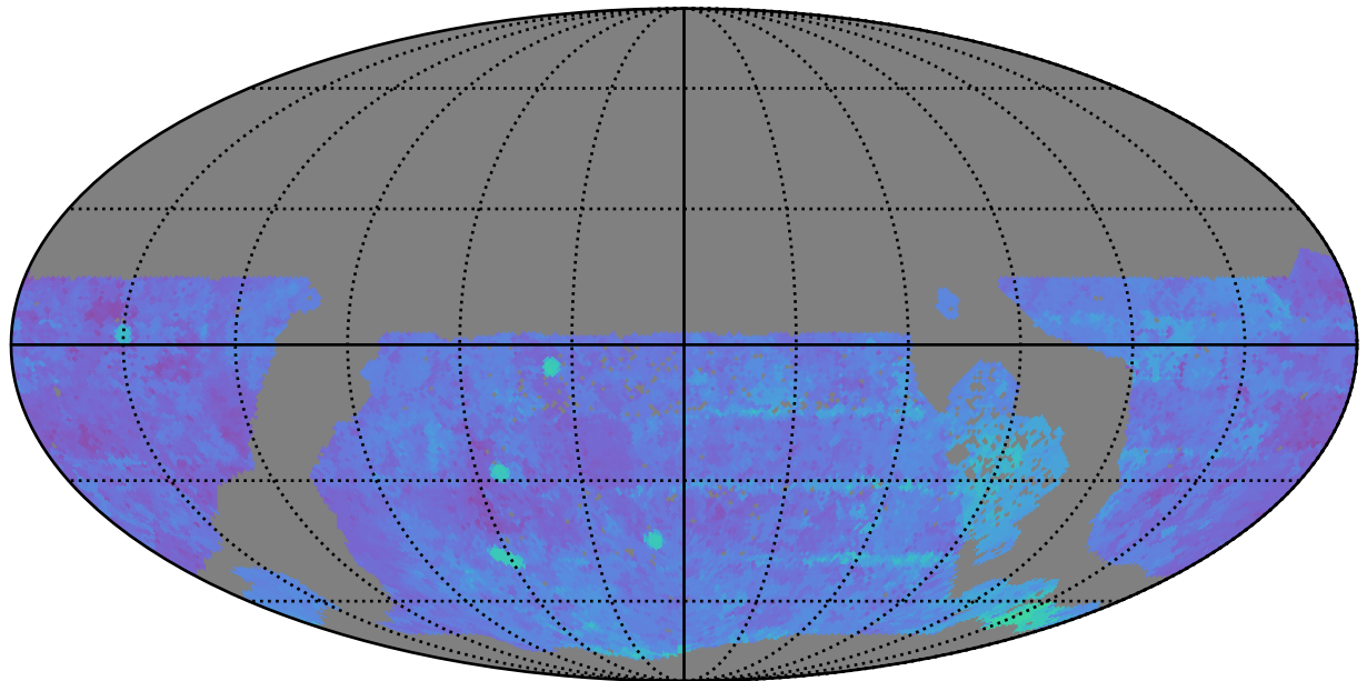
ddf_acor_sf20_lsf0_lsr0_v3.4_10yrs WFD g band: 80thPercentile Season Length
