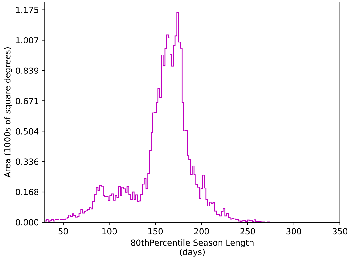
ddf_acor_sf20_lsf0_lsr0_v3.4_10yrs All sky z band: 80thPercentile Season Length
