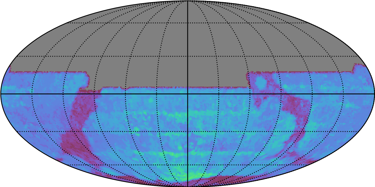
ddf_acor_sf20_lsf0_lsr0_v3.4_10yrs All sky y band: 80thPercentile Season Length
