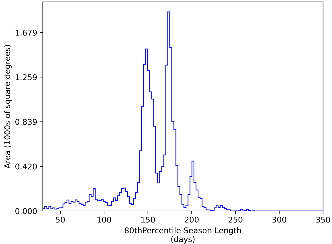
ddf_acor_sf20_lsf0_lsr0_v3.4_10yrs All sky y band: 80thPercentile Season Length
