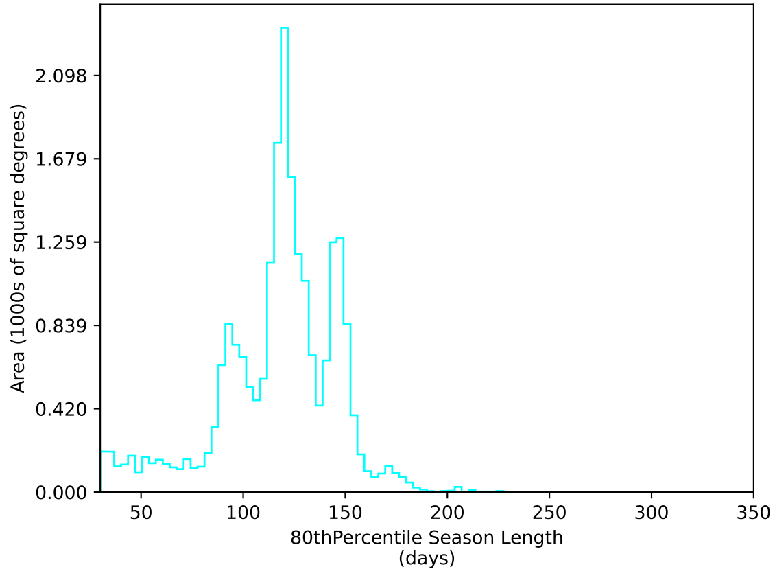
ddf_acor_sf20_ls0_lsr0_v3.4_10yrs All sky u band: 80thPercentile Season Length
