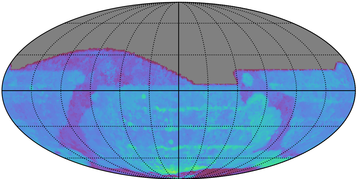
ddf_acor_sf20_lsf0_lsr0_v3.4_10yrs All sky r band: 80thPercentile Season Length
