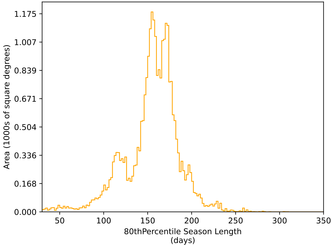
ddf_acor_sf20_lsf0_lsr0_v3.4_10yrs All sky r band: 80thPercentile Season Length
