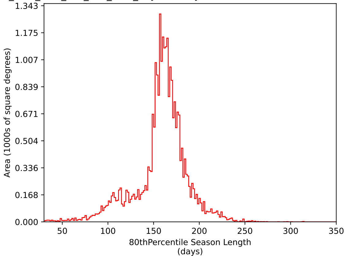
ddf_acor_sf20_lsf0_lsr0_v3.4_10yrs All sky i band: 80thPercentile Season Length
