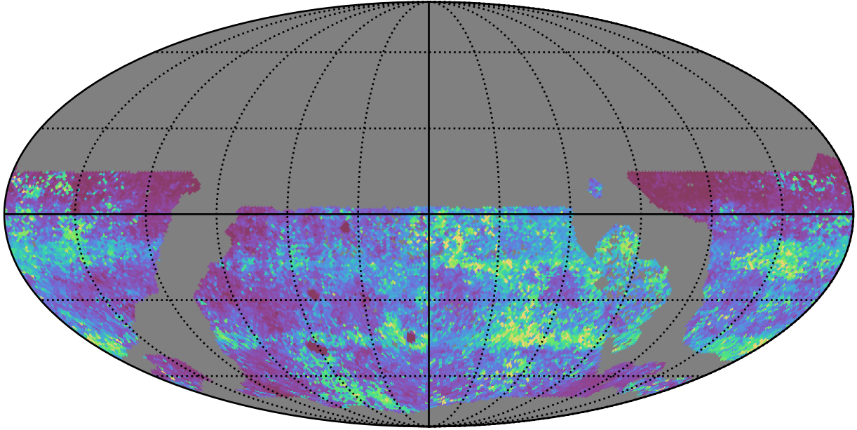
ddf_acor_sf20_lsr0_v3.4_10yrs WFD zy bands: 75th Percentile Intranight Timespan
