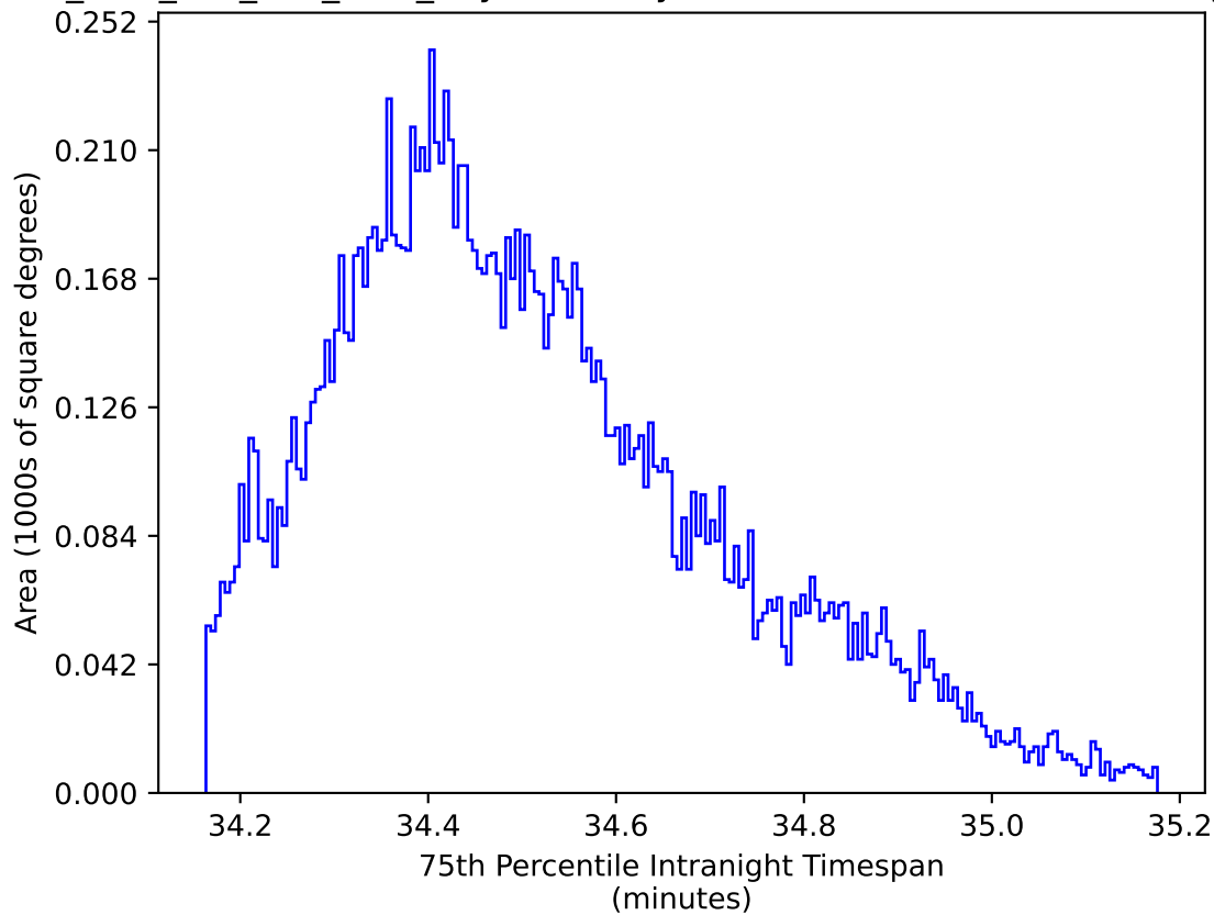
ddf_acor_sf20_lsf0_lsr0_v3.4_10yrs WFD zy bands: 75th Percentile Intranight Timespan
