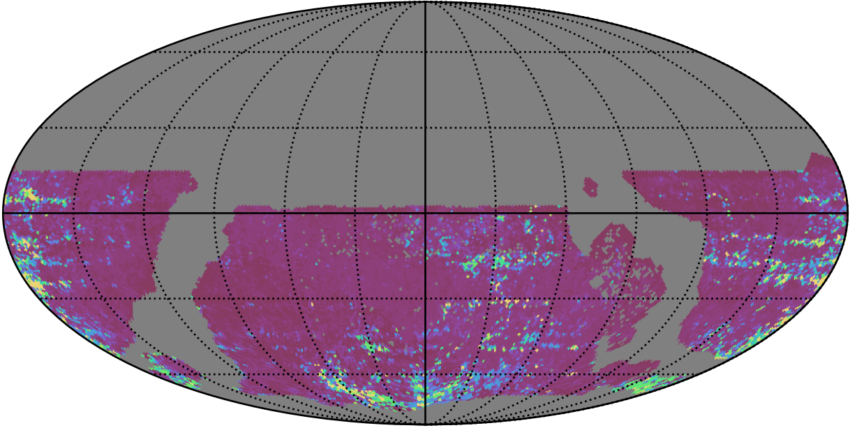
ddf_acor_sf20_lsf0_lsr0_v3.4_10yrs WFD z band: 75th Percentile Intranight Timespan
