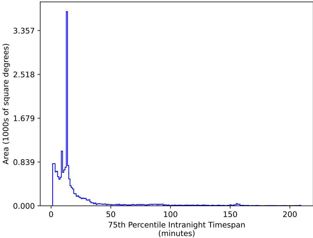
ddf_acor_sf20_lsf0_lsr0_v3.4_10yrs WFD z band: 75th Percentile Intranight Timespan
