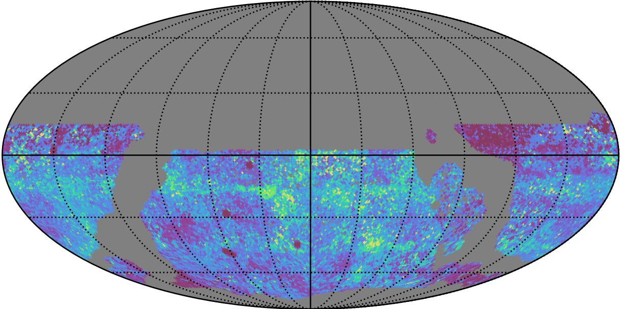
ddf_acor_sf20_lsf0_lsr0_v3.4_10yrs WFD y band: 75th Percentile Intranight Timespan
