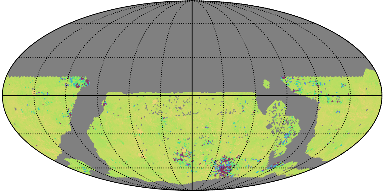
ddf_acor_sf20_lsf0_lsr0_v3.4_10yrs WFD ug bands: 75th Percentile Intranight Timespan
