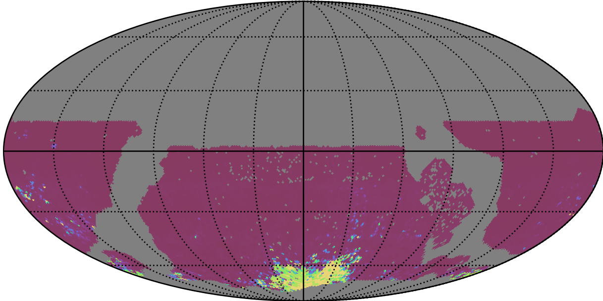
ddf_acor_sf20_lsf0_lsr0_v3.4_10yrs WFD ri bands: 75th Percentile Intranight Timespan
